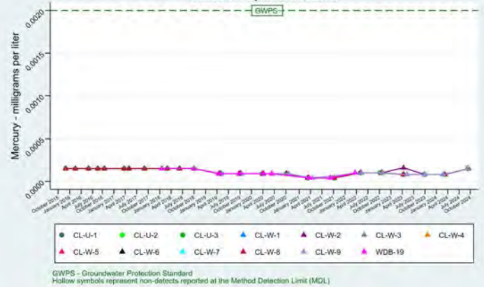
Mercury - Time Series Intermountain Power Service Corporation - Intermountain Generation Facility Combustion By-Products Landfill
