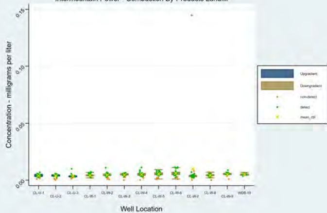
Molybdenum - Box Plots Intermountain Power - Combustion By-Products Landfill
