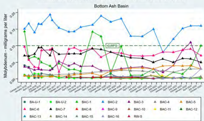
Molybdenum - Time Series Intermountain Power Service Corporation - Intermountain Generation Facility
