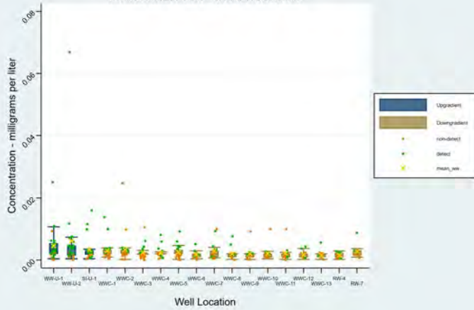
Chromium - Box Plots Intermountain Power - Waste Water Basin
