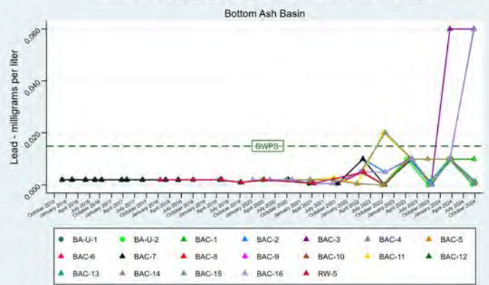
Lead - Time Series Intermountain Power Service Corporation - Intermountain Generation Facility
