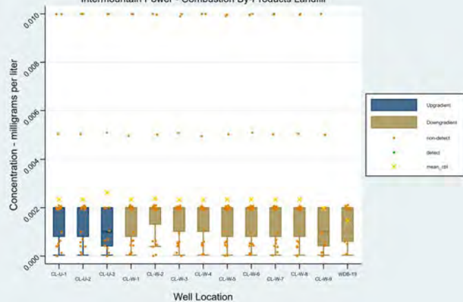
Lead - Box Plots Intermountain Power - Combustion By-Products Landfill
