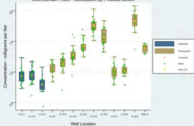
Fluoride - Box Plots Intermountain Power - Combustion By-Products Landfill
