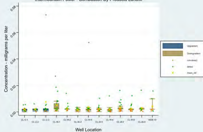
Chromium - Box Plots Intermountain Power - Combustion By-Products Landfill
