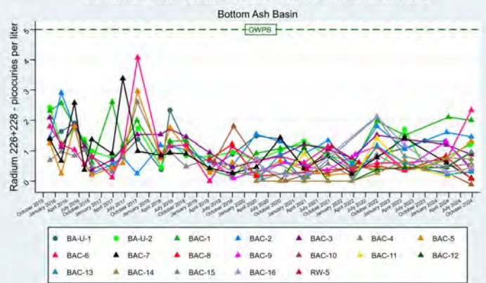
Radium 226+228 - Time Series Intermountain Power Service Corporation - Intermountain Generation Facility
