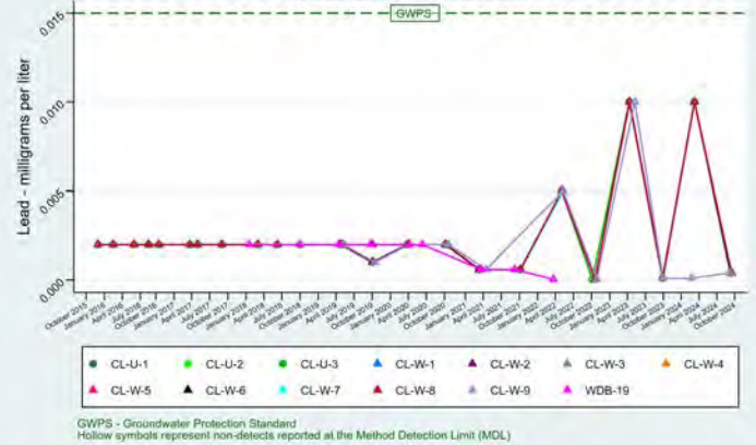
Lead - Time Series Intermountain Power Service Corporation - Intermountain Generation Facility Combustion By-Products Landfill
