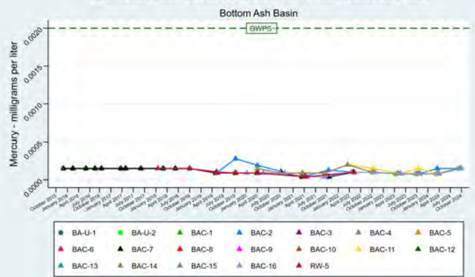
Mercury - Time Series Intermountain Power Service Corporation - Intermountain Generation Facility
