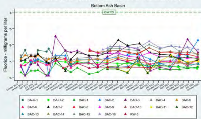
Fluoride - Time Series Intermountain Power Service Corporation - Intermountain Generation Facility
