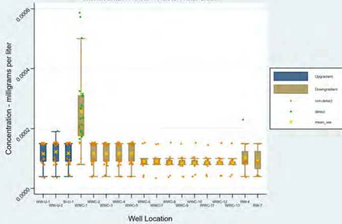
Mercury - Box Plots Intermountain Power - Waste Water Basin
