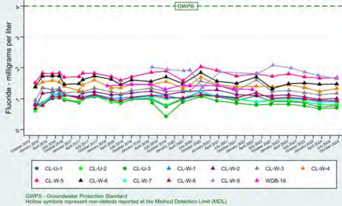
Fluoride - Time Series Intermountain Power Service Corporation - Intermountain Generation Facility Combustion By-Products Landfill
