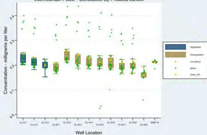
Lithium - Box Plots Intermountain Power - Combustion By-Products Landfill
