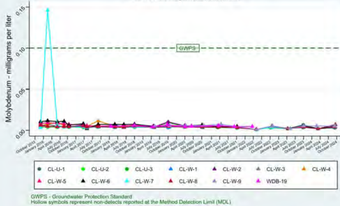
Molybdenum - Time Series Intermountain Power Service Corporation - Intermountain Generation Facility Combustion By-Products Landfill
