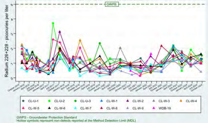
Radium 226+228 - Time Series Intermountain Power Service Corporation - Intermountain Generation Facility Combustion By-Products Landfill
