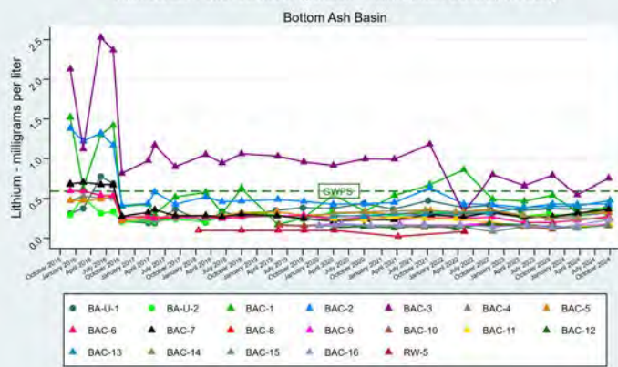
Lithium - Time Series Intermountain Power Service Corporation - Intermountain Generation Facility
