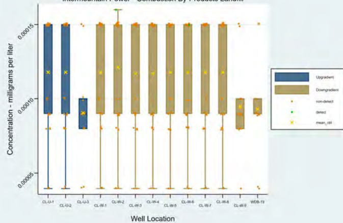
Mercury - Box Plots Intermountain Power - Combustion By-Products Landfill
