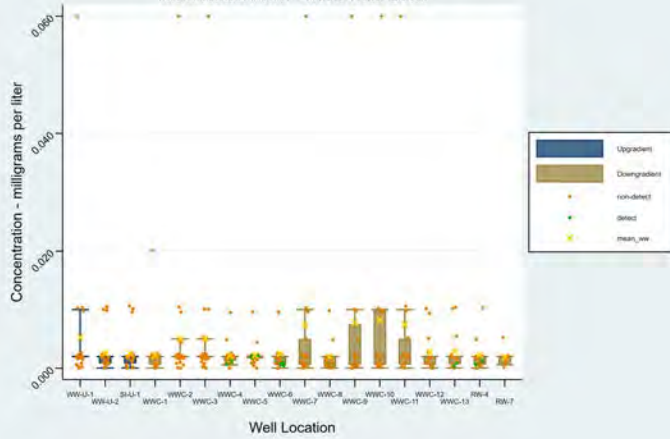
Lead - Box Plots Intermountain Power - Waste Water Basin
