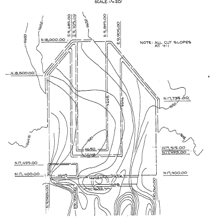
PRELIMINARY GRADING DETAIL ASH WATER RECYCLE BASIN SCALE: 1"=100'
