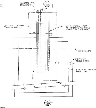
TYPE 4 SYNTHETIC LINER PIPE PENETRATION SCALE: 1/4"=1'-0"
