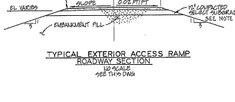
TYPICAL EXTERIOR ACCESS RAMP ROADWAY SECTION 10\"/>
