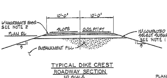
TYPICAL DIKE CREST ROADWAY SECTION 10\"/>
