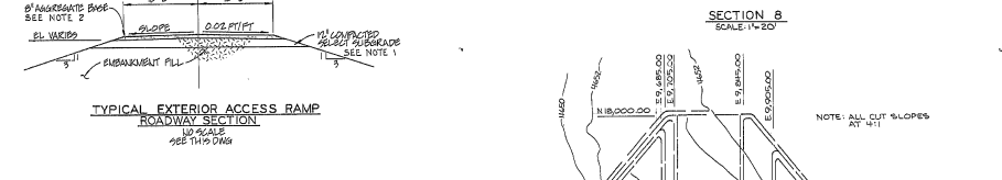
TYPICAL EXTERIOR ACCESS RAMP ROADWAY SECTION 10" SCALE SEE THIS DWG
