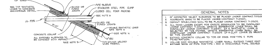
TYPICAL SYNTHETIC LINER PIPE PENETRATION DETAIL TYPE 1 & 2 NO SCALE
