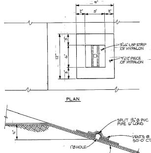
HYALON GAS VENT DETAIL NO SCALE SEE THIS DWG
