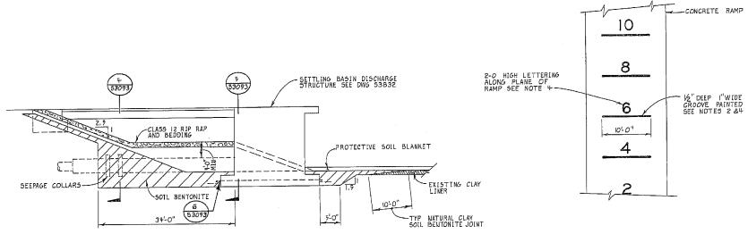
SETTLING BASIN STRUCTURE DIKE INTERFACE SCALE: 1/4\"/>
