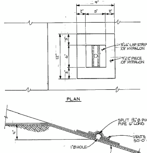
HYPALON GAS VENT DETAIL NO SCALE SEE THIS DWG
