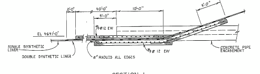
SECTION 1 NO SCALE SEE THIS DWG
