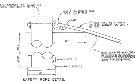
SAFETY ROPE DETAIL NO SCALE
