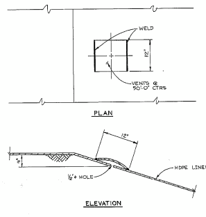
HDPE GAS VENT DETAIL NO SCALE SEE THIS DWG
