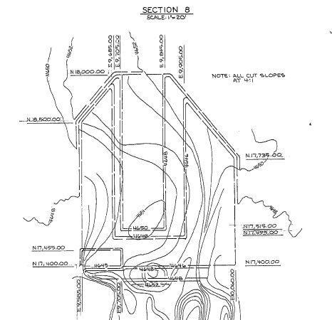
PRELIMINARY GRADING DETAIL ASH WATER RECYCLE BASIN SCALE: 1"=100'
