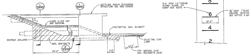
SETTLING BASIN STRUCTURE DIKE INTERFACE SCALE: 1/4\"/>
