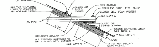
TYPICAL SYNTHETIC LINER PIPE PENETRATION DETAIL TYPE 1 & 2 NO SCALE
