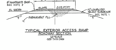
TYPICAL EXTERIOR ACCESS RAMP ROADWAY SECTION 10" SCALE SEE THIS DWG
