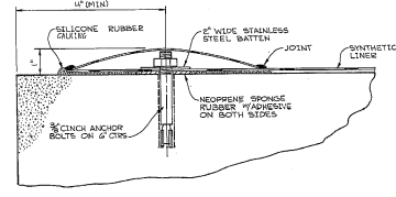
TYPICAL SYNTHETIC LINER TO CONCRETE ANCHORAGE DETAIL SCALE: 1"=10'
