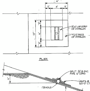
HYPALON GAS VENT DETAIL NO SCALE SEE THIS DWG
