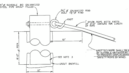
SAFETY ROPE DETAIL NO SCALE
